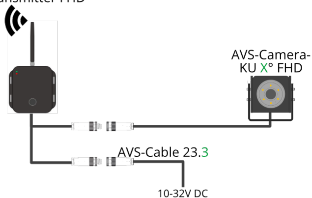
AVS-Wireless Transmitter FHD
